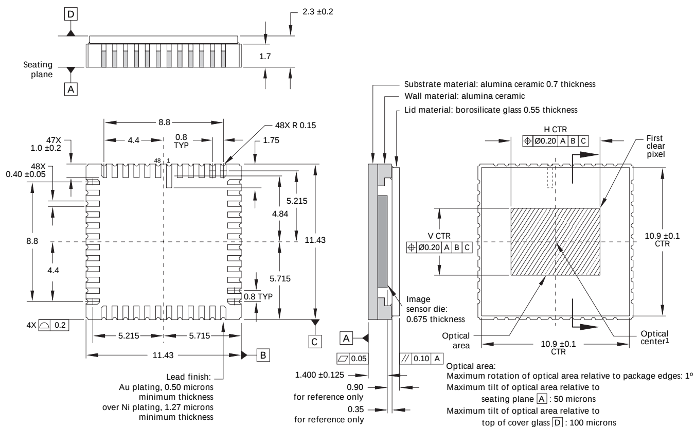
Figure 23: 48-Pin CLCC Package
