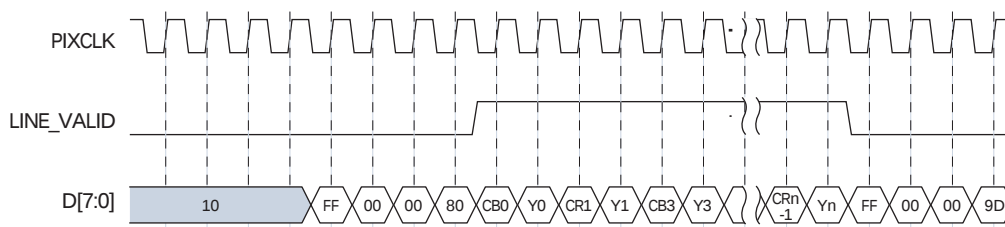
Figure 12: Horizontal Timing
