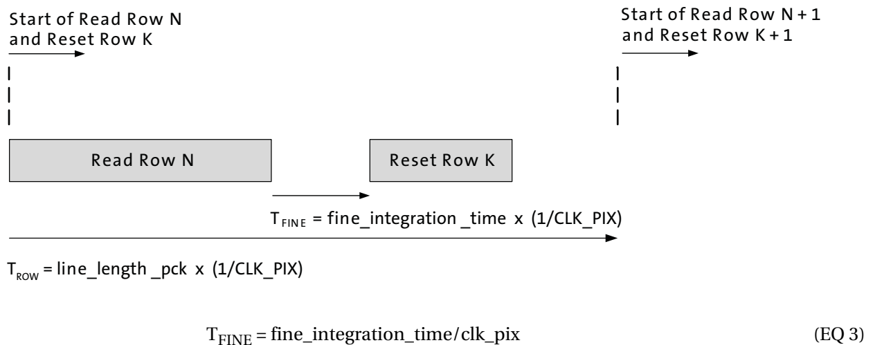
Figure 17: Row Read and Row Reset Showing Fine Integration
