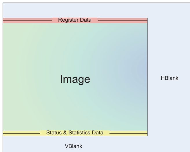
Figure 36: Frame Format with Embedded Data Lines Enabled
