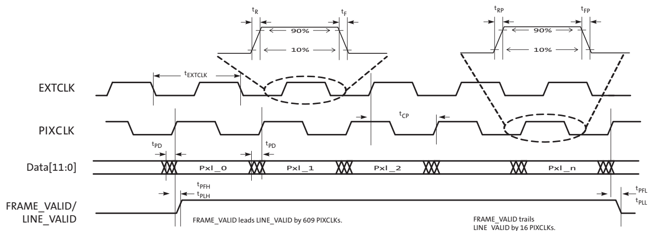
Figure 45: I/O Timing Diagram
