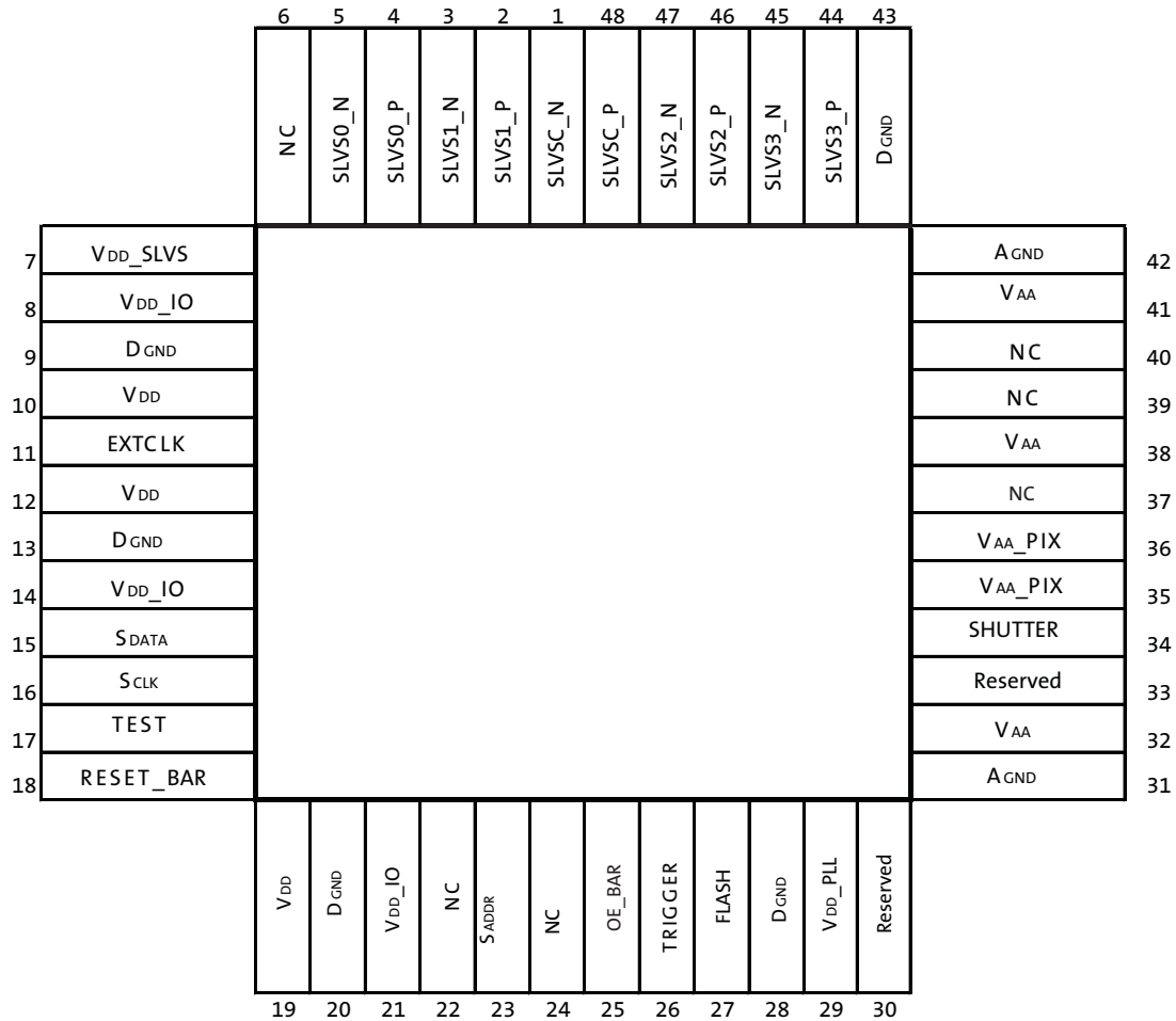
Figure 5: 48 iLCC Package, HiSpi Output
