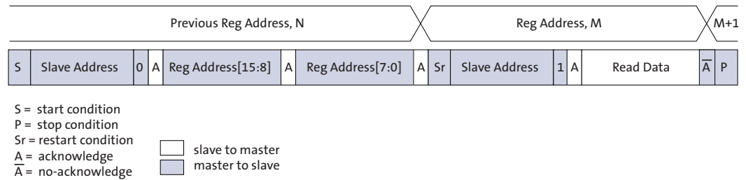
Figure 21: Single READ from Random Location
