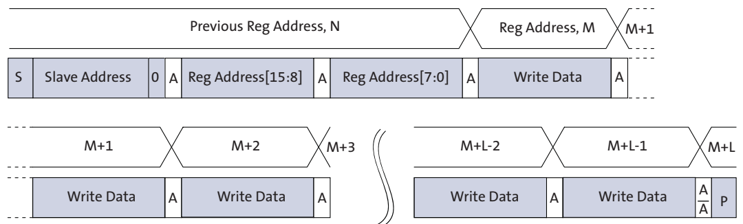
Figure 26: Sequential WRITE, Start at Random Location
