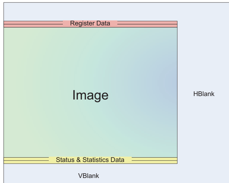
Figure 19: Frame Format with Embedded Data Lines Enabled
