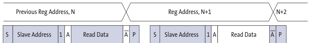
Figure 22: Single READ from Current Location
