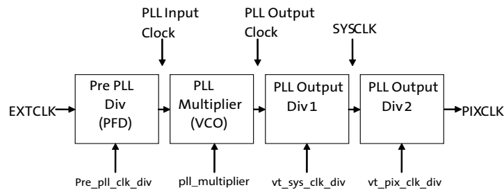
Figure 16: PLL-Generated Master Clock PLL Setup
