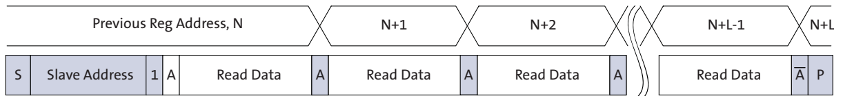
Figure 24: Sequential READ, Start from Current Location
