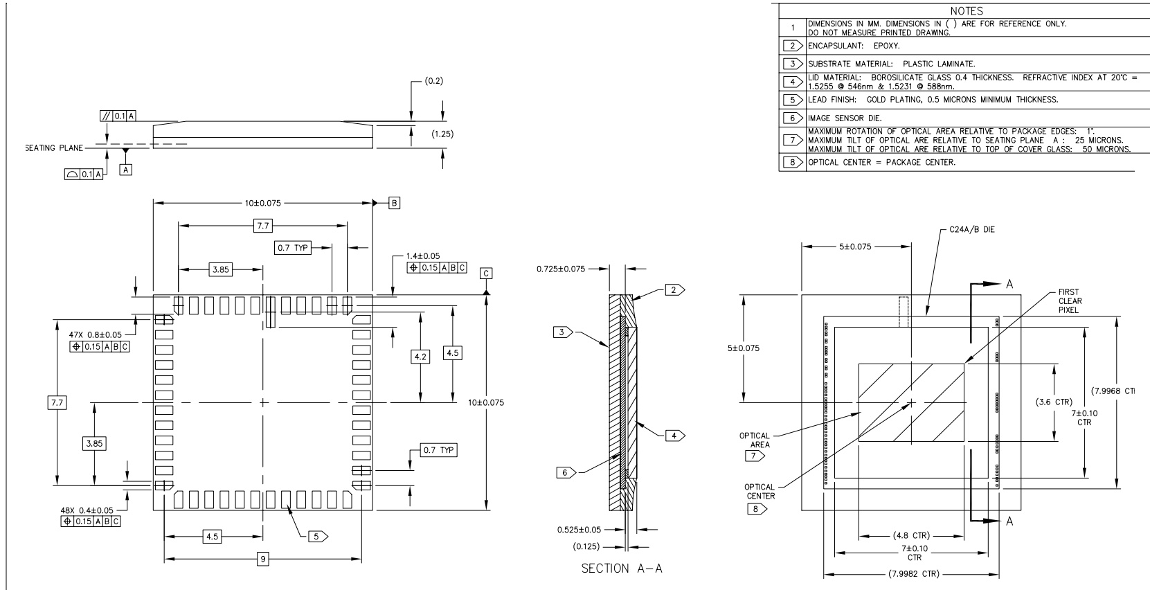
Figure 36: 48 iLCC Package Outline Drawing
