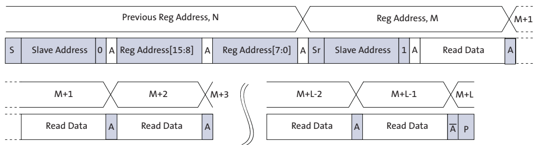
Figure 23: Sequential READ, Start from Random Location
