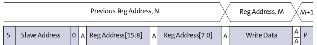
Figure 25: Single WRITE to Random Location
