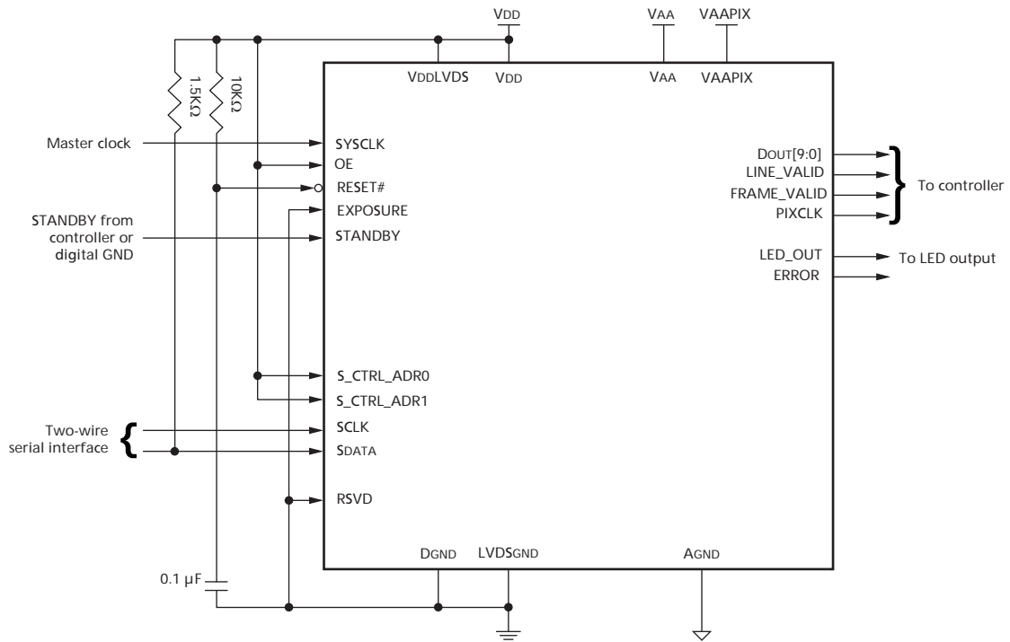
Figure 1: Typical Configuration (Connection) Parallel Output Mode
