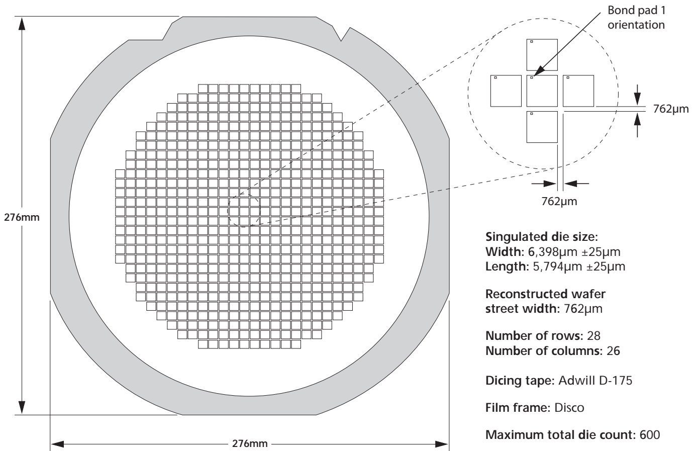
Figure 3: MTV032 Die Orientation in Reconstructed Wafer
