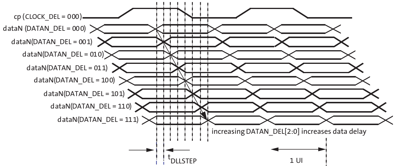
Figure 11: Delaying Data with Respect to the Clock
