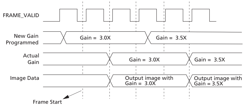
Figure 24: Latency of Analog Gain Change When AGC Is Disabled
