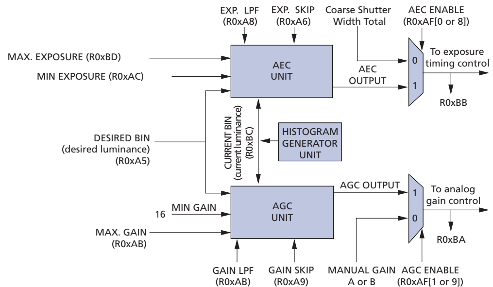
Figure 27: Controllable and Observable AEC/AGC Registers
