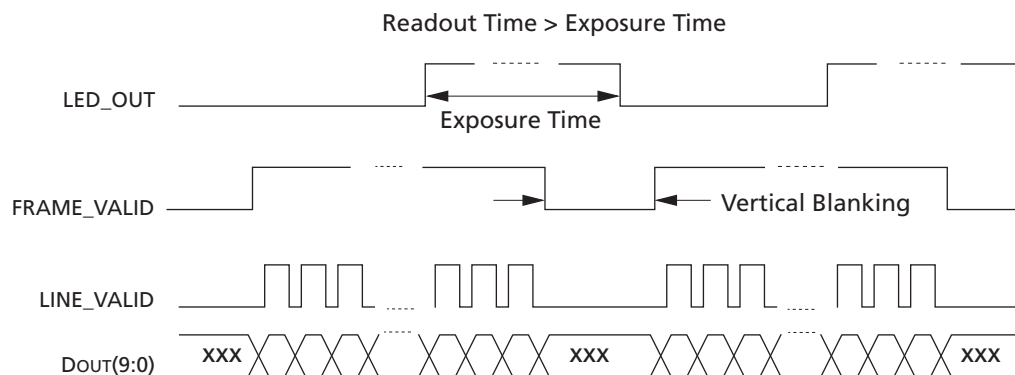
Figure 14: Simultaneous Master Mode Synchronization Waveforms #2
