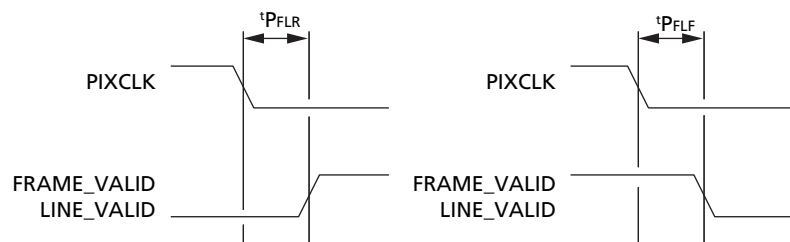
Figure 37: Propagation Delays for FRAME_VALID and LINE_VALID Signals
