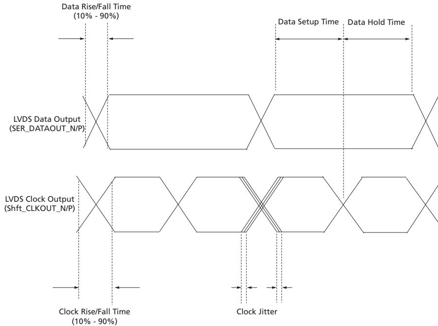
Figure 35: LVDS Timing
