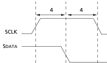
Figure 39: Serial Host Interface Start Condition Timing
