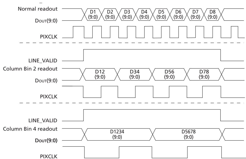
Figure 31: Readout of 8 Pixels in Normal and Column Bin Output Mode
