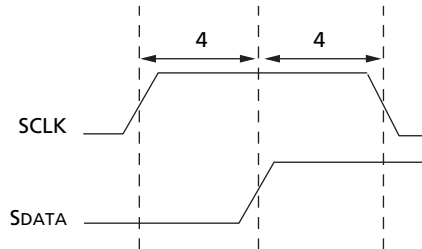
Figure 40: Serial Host Interface Stop Condition Timing
