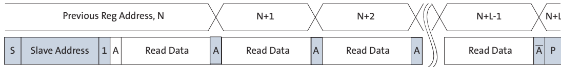
Figure 7: Sequential READ, Start from Current Location
