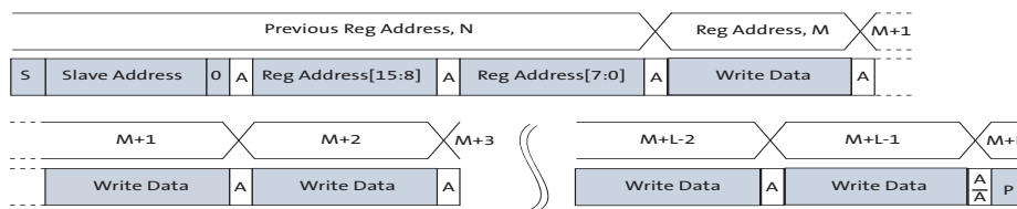
Figure 9: Sequential Write, Start at Random Location
