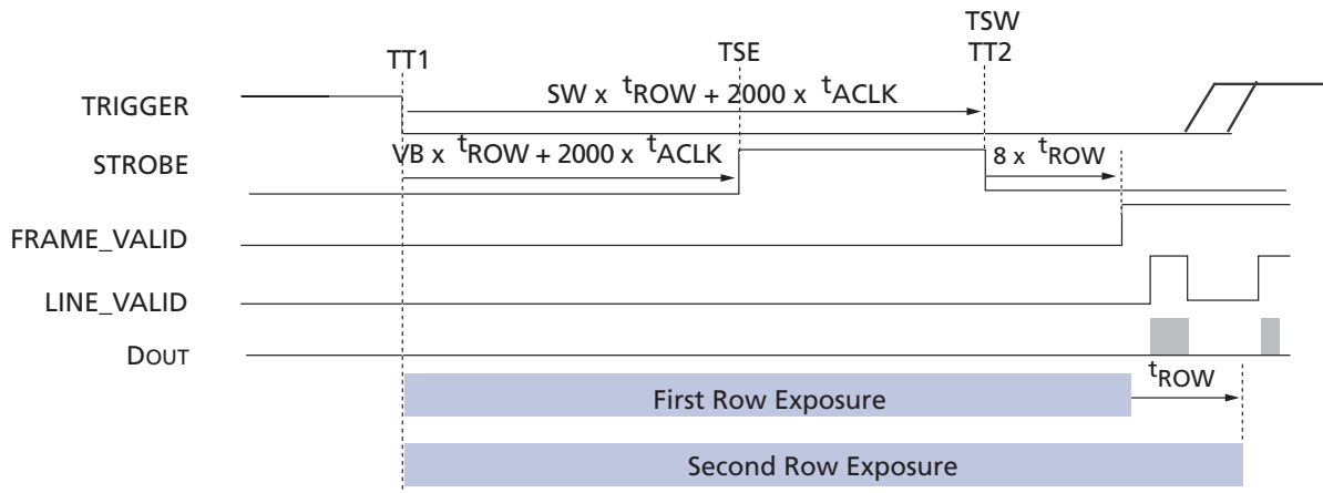
Figure 2: Master Mode GRR Timing
