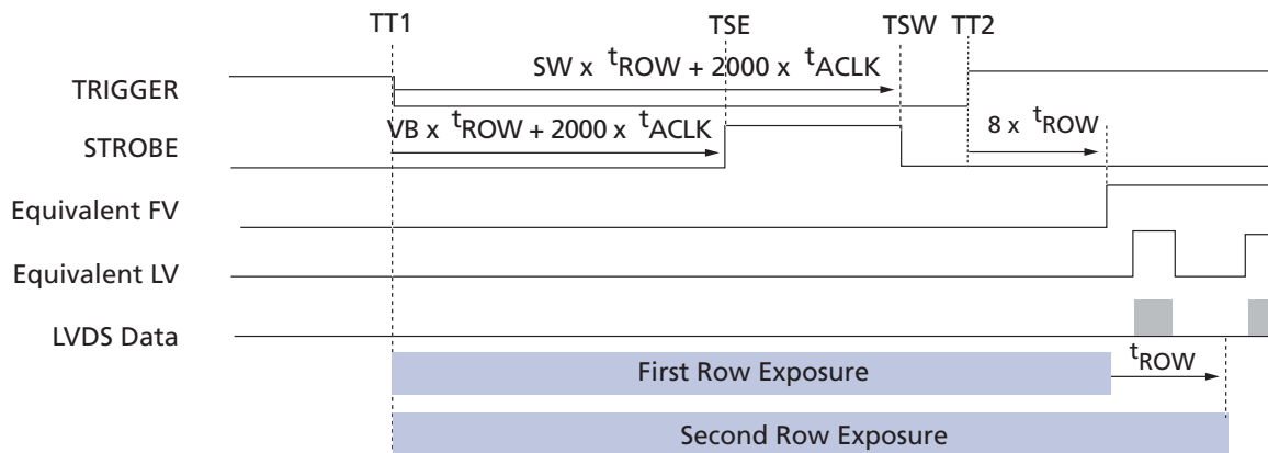
Figure 3: Slave Mode GRR Timing
