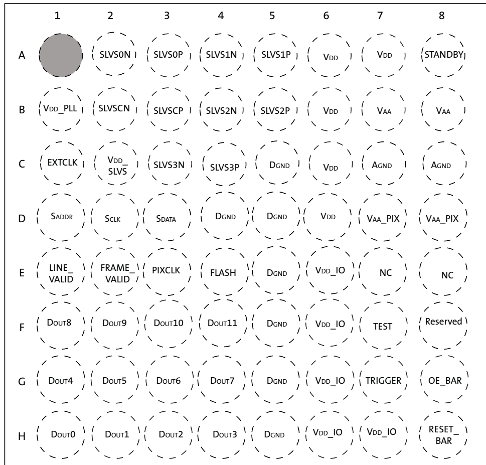
Figure 4: 9 x 9 mm 64-Ball IBGA Package, Parallel Output
