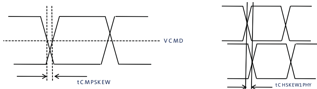
Figure 32: Skew Within the PHY and Output Channels
