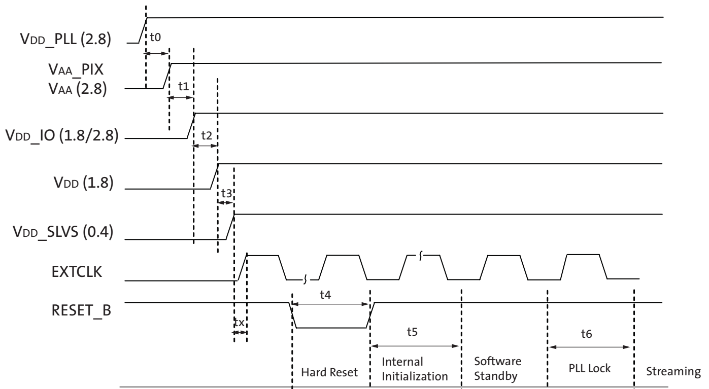
Figure 33: Power Up
