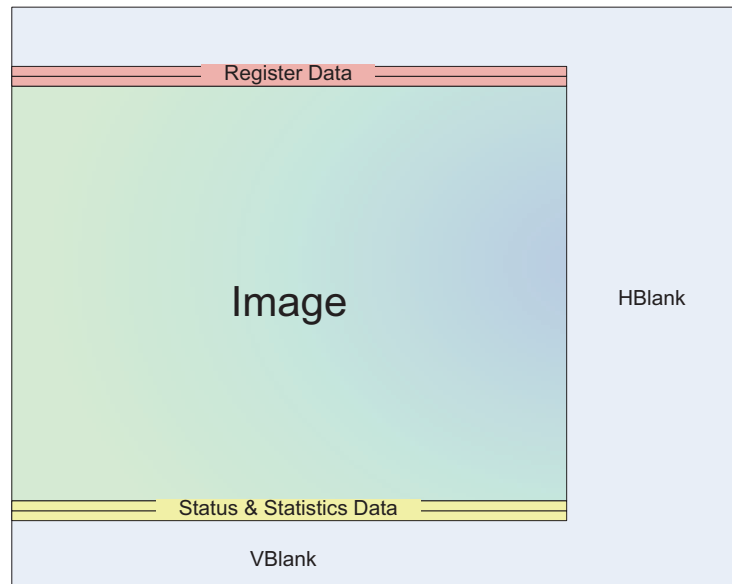
Figure 18: Frame Format with Embedded Data Lines Enabled
