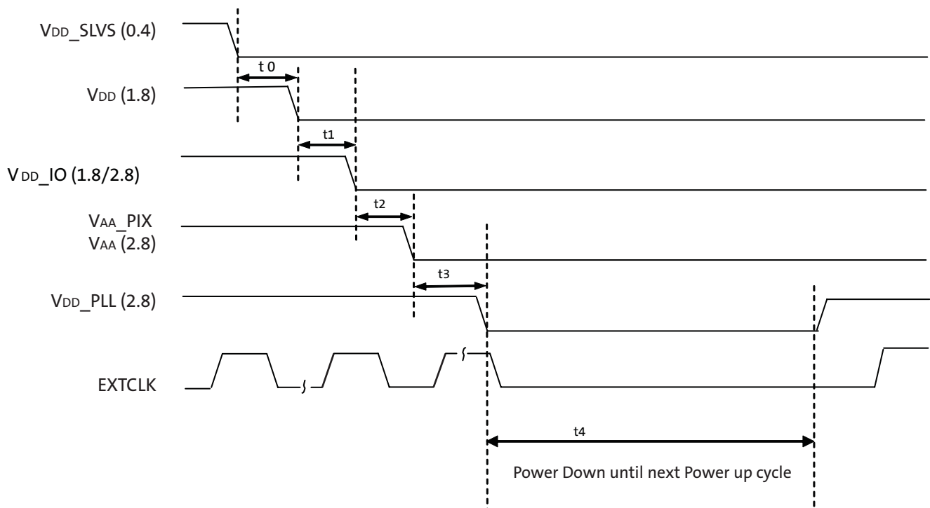
Figure 34: Power Down
