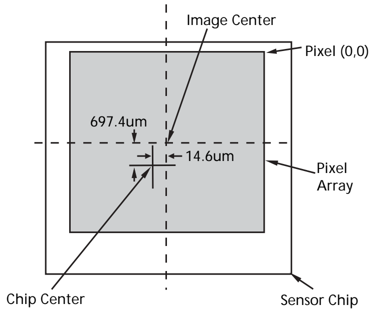
Figure 29: Image Center Offset
