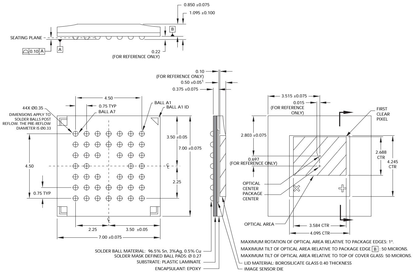
Figure 30: 44-Ball iBGA Package Outline Drawing
