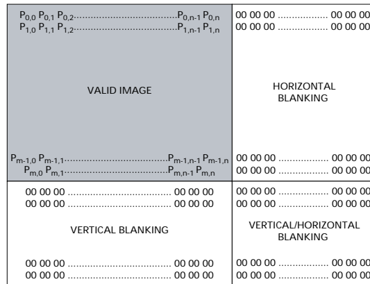
Figure 6: Spatial Illustration of Image Readout
