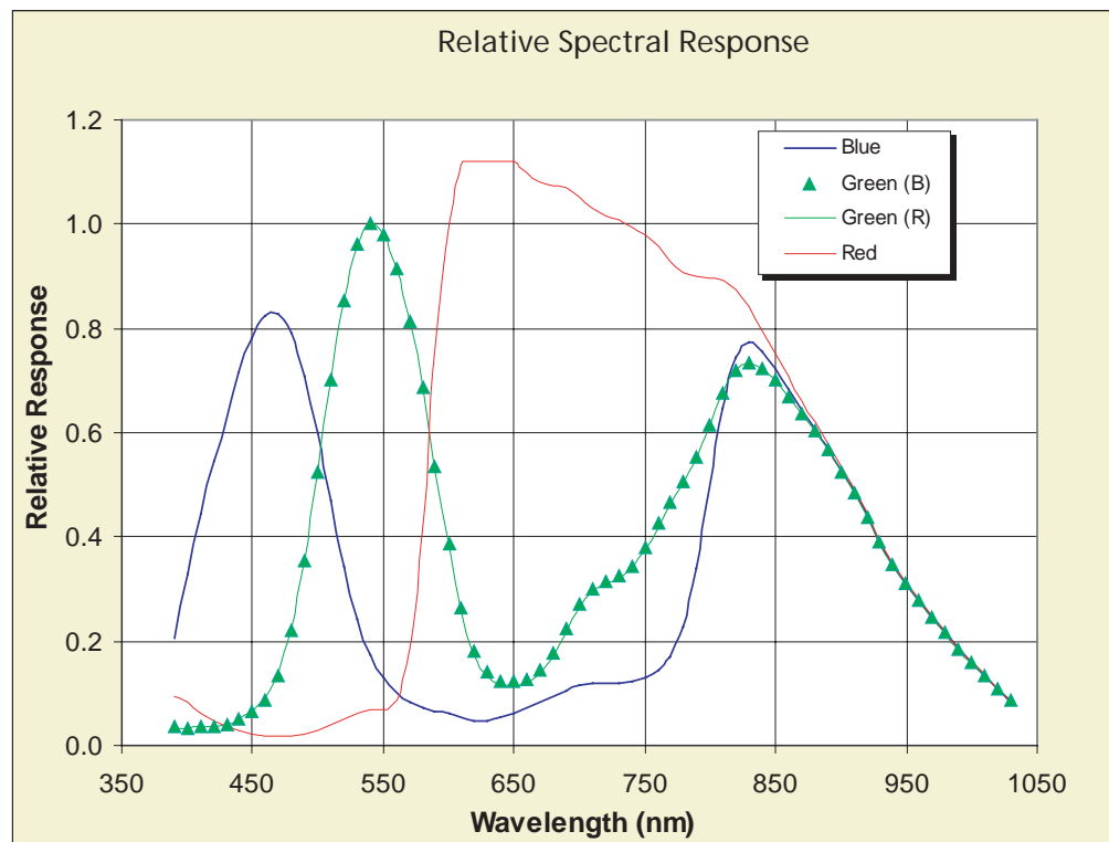
Figure 28: Spectral Response
