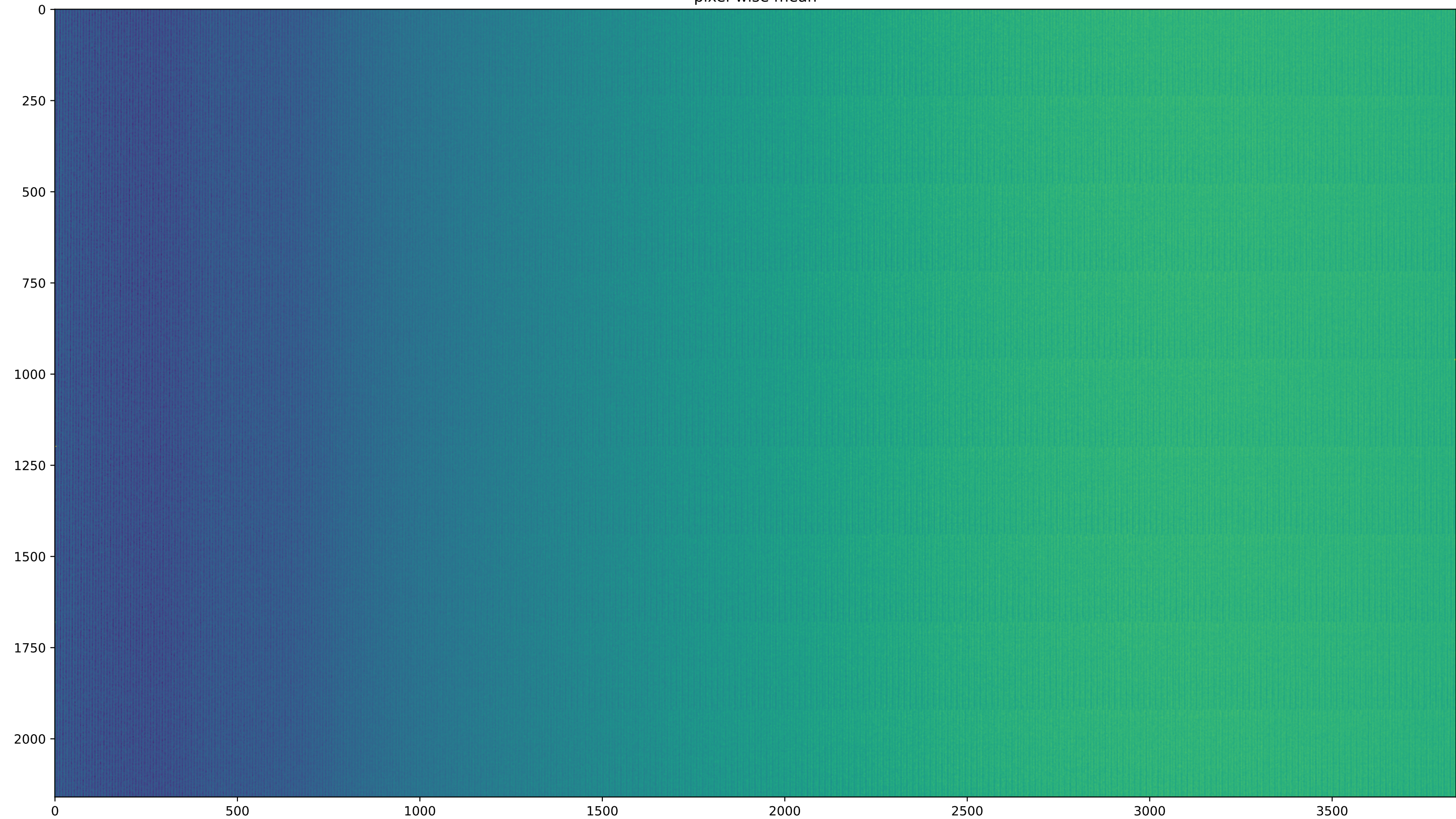
pixel-wise mean
